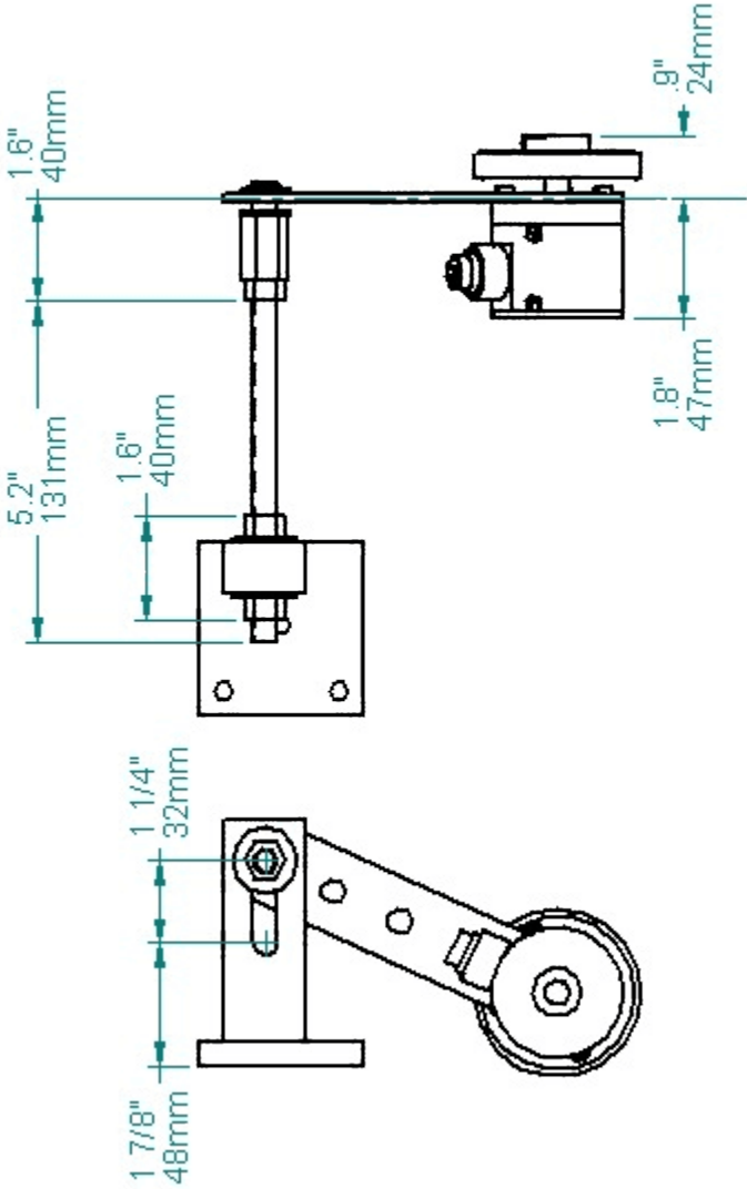
R21 with measuring wheels and MB-UB2 mounting hardware
